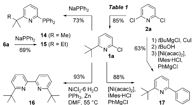
Scheme 1. Efficient entries into the synthesis of ligands for transition metals or heterocyclic building blocks by a copper-catalyzed tertiary butylation of 2,6-dichloropyridine ( 2a ). IMes·HCl = 1,3-bis(2,4,6-trimethylphenyl)imidazolium chloride.
