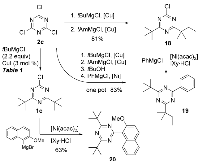
Scheme 2. Elaboration of triazine building blocks from 2c . IXy·HCl = 1,3-bis(2,6-dimethylphenyl)imidazolium chloride. [30]
